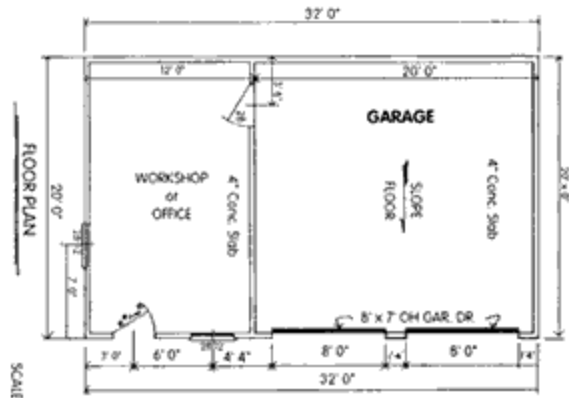
20' W x 32' L 'STRATFORD' 2 CAR GARAGE Dad's Retreat, a 12' x 20' workshop with a 20' x 20' garage all in one.
