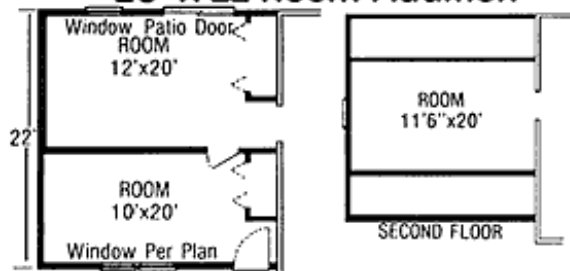
20' x 22 Room Addition
